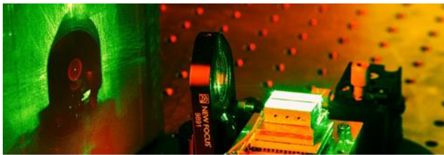
Source of entangled photons: spontaneous parametric down conversion in a non-linear crystal. (©Fraunhofer IPM)
