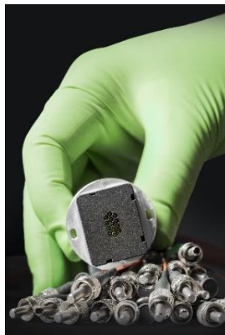
Without the image sensor, the 39 spectra can be seen at the output of the optics. © Fraunhofer IOF
